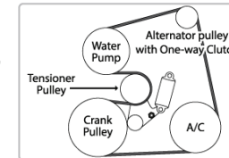
ENGINE ZD30D15 WITH 7PK AUTO-TENSIONED DRIVE BELT SYSTEM.
