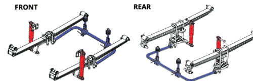
PARABOLIC LEAF SPRING WITH DUAL ACTING SHOCK ABSORBER + STABILIZER BAR
